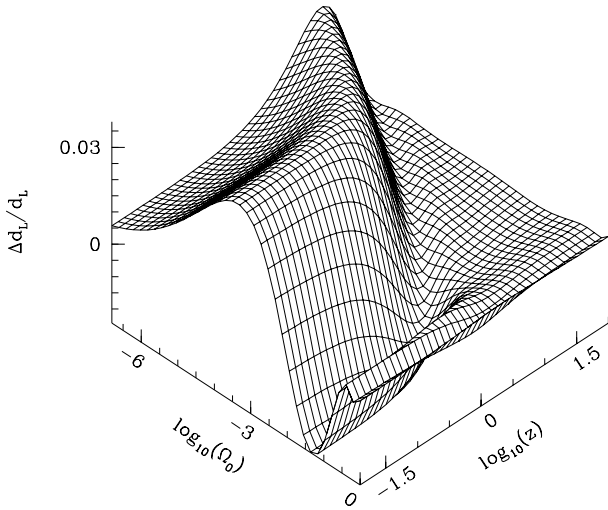
FIG. 1.—Global error surface. Our minmax fit minimized all errors for \log_{10} \Omega_0 \geq -0.7 , where the error is less than 0.4% for all redshifts.
