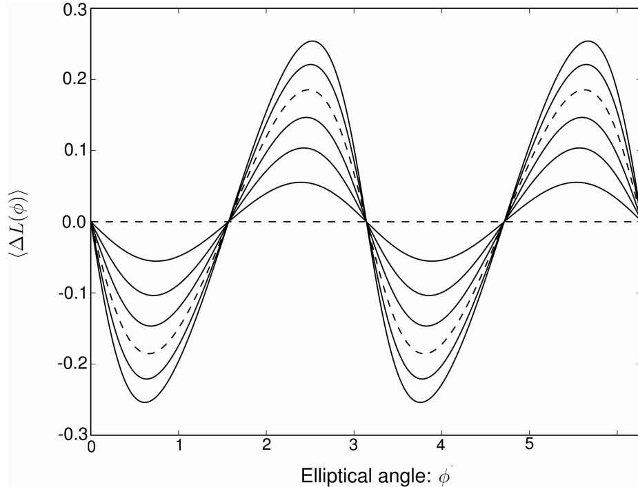
Figure 3.5: Plot of \langle \Delta L(\phi) \rangle for various aspect ratios as a function of the elliptical parameter \phi . With area fixed at E_a E_b \pi = 1 , aspect ratios are plotted from k = E_a/E_b = 1 to k = 2 in increments of 1/6 . The dashed lines indicate the two curves k = 1, 5/3 , with the flat line corresponding to the circle.
