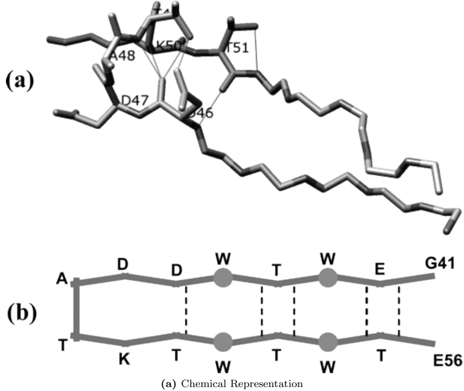
Figure 4.3: Native state of the trzip4-m1 peptide represented schematically. This image was generated from the NMR structure of trzip4 (PDB code 1LE3, structure 1). The dashed lines represent the hydrogen bonds. Image used with permission from Gai. 3
