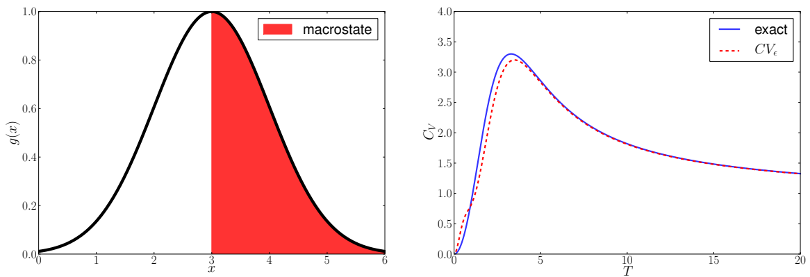
Figure A.3: CV_\epsilon with \epsilon = 1/2 . 50.0% of g(x) is considered as a single macrostate (see text for details).
