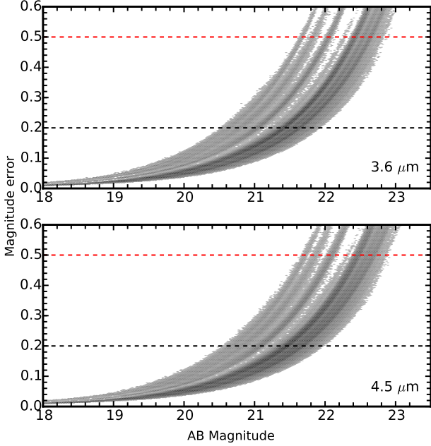
FIG. 14.— Estimation of the SpIES detection limit at 3.6\,\mu\text{m} (top) and 4.5\,\mu\text{m} (bottom). The grey points indicate the error in magnitude vs. magnitude. The 5\sigma limit occurs at a magnitude error of 0.2 (black dashed line), and the 2\sigma limit occurs at a magnitude error of 0.5 (red dashed line). These values are determined by propagating the error in the expression for magnitude, resulting in the ratio of noise to signal as the error in magnitude. The intersection of the right edge of the grey points with the respective magnitude error is the approximate detection threshold. Differences in shading indicates the density of points.
