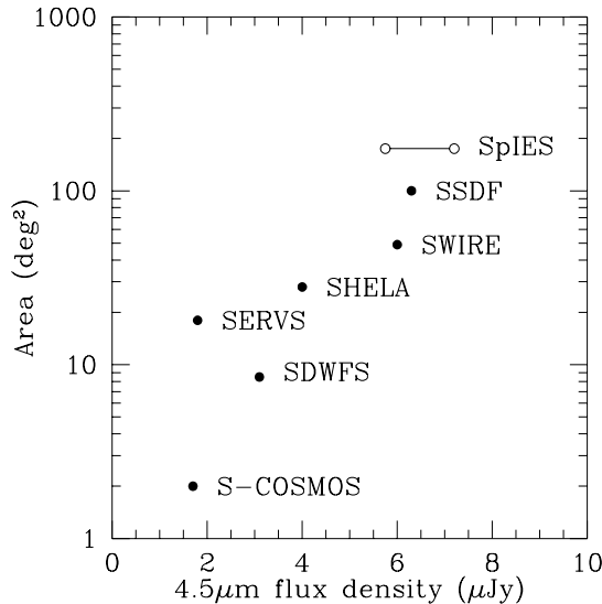
FIG. 3.— Comparison of the calculated 4.5 \mu\text{m} 5\sigma depth to area of the major Spitzer surveys. Depths are calculated using the Spitzer Sensitivity Performance Estimation Tool (SENS-PET) assuming a low background. At \sim 115 \text{ deg}^2 in area SpIES is the largest Spitzer survey and probes SWIRE depths (Lonsdale et al. 2003). Open circles show the measured depth (left; see Table 9) and calculated depth from SENS-PET with a medium background (right) for SpIES.
